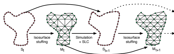
Figure 2: Each time step uses one surface triangulation and one tetrahedral mesh. A new time step's surface S_{t+1} is created by semi-Lagrangian advection: tracing paths backward in time through the velocity field on M_t to locate a point relative to S_t . The isosurface stuffing algorithm generates a tetrahedral mesh M_{t+1} (with coarser surface resolution) from S_{t+1} . Velocities are interpolated/extrapolated from M_t .
